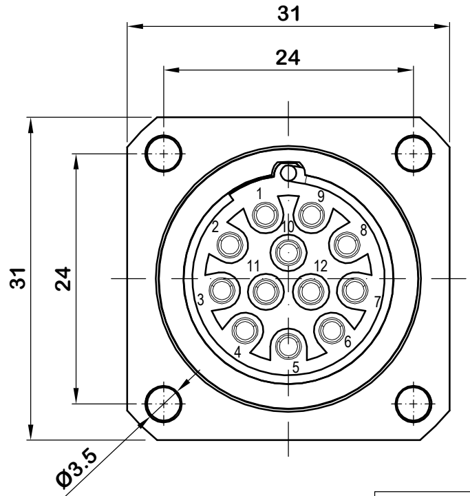
General dimensions (mm) Scale 2:1
