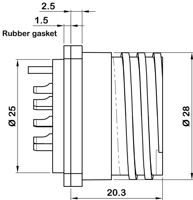
General dimensions (mm) Scale 2:1
