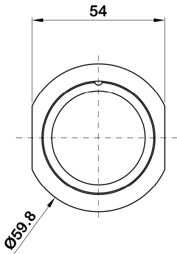
Side to assemble MALE plugs / extenders
